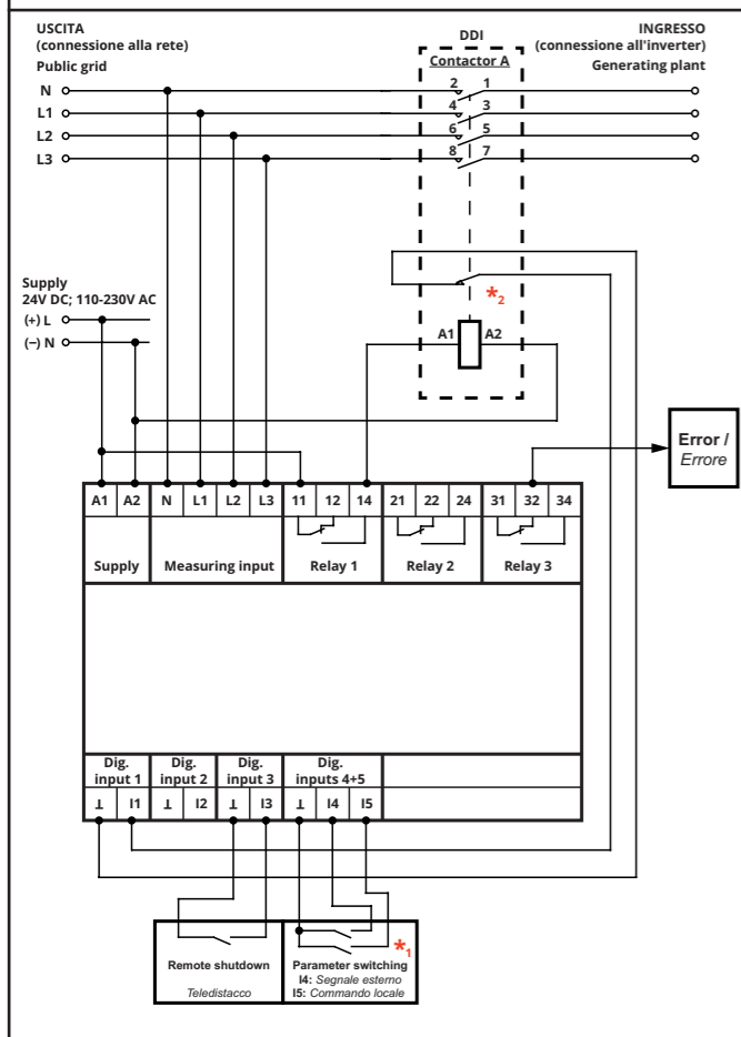
Connection diagram 2:
