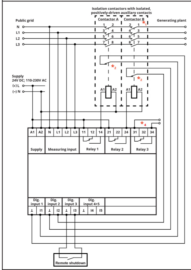
Connection diagram 1:
