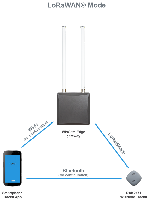
Figure 2: LoRaWAN mode
