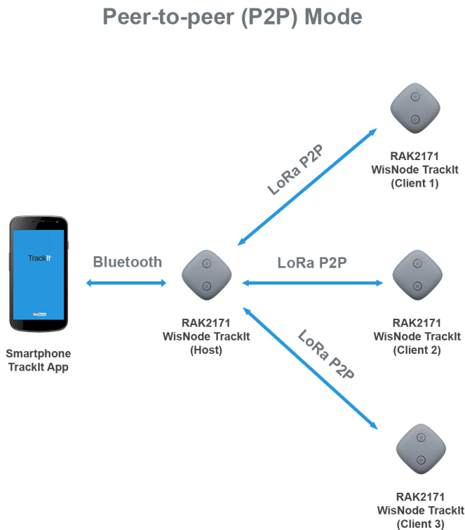
Figure 12: P2P mode
