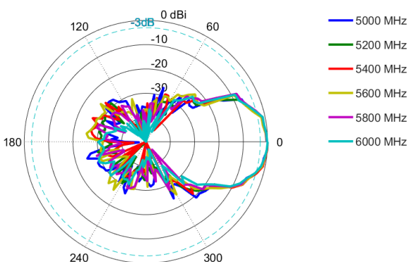
Elevation: 5000 – 6000 MHz
