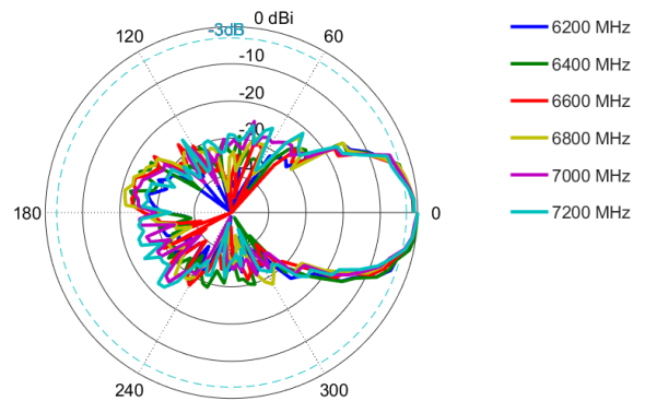
Elevation: 6200 – 7200 MHz
