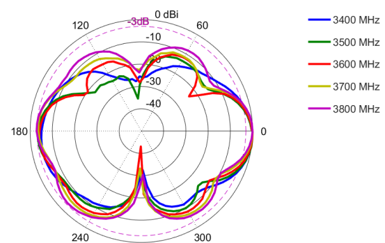
Elevation1 (Side View): 3400–3800 MHz
